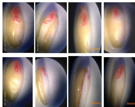
V7 : Villemur/3/Lahn//Gs/Stk/Dra2/Bcr/5/Lks4 /4/ ...
