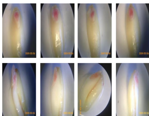
V9: Lahaucan
