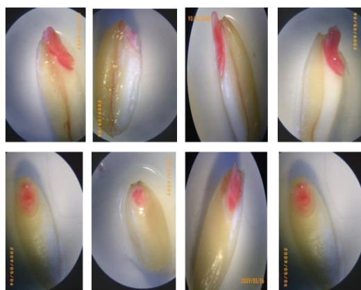
V6 : Azeghar-1/6/Zna-1/5Awal1/4/Ruff//Jo/Cr/3/F9.3
