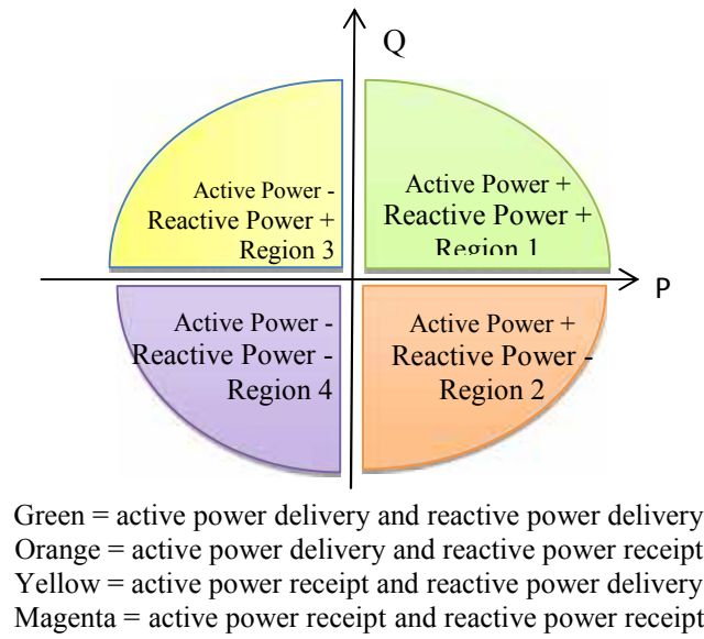
Figure 3 : P-Q characteristics of a VSC-HVDC system
