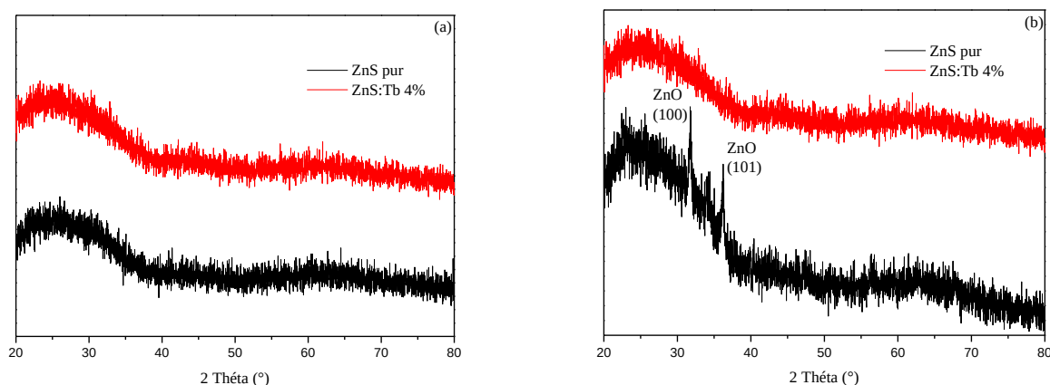
Fig.1. X-ray diffraction of \text{ZnS:Tb}^{3+} thin films (0-4%), a) before annealing, b) after annealing (500 ° C, 1h).
