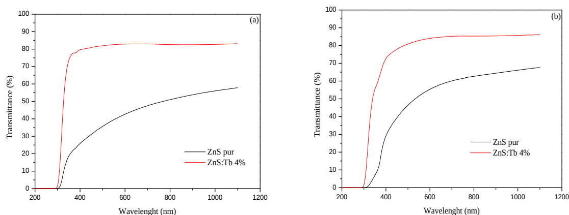
Fig.4: Transmittance spectra of ZnS:Tb 3+ thin films (0-4%), (a) before annealing, (b) after annealing (1H, 500°C).
