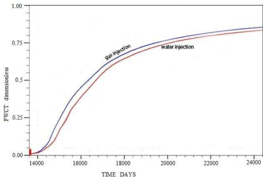
Figure.6. Comparison of Production Water Cut for Two Scenarios.
