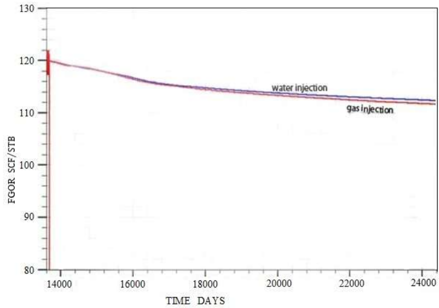
Figure.5. Comparison of Production GOR for Two Scenarios.
