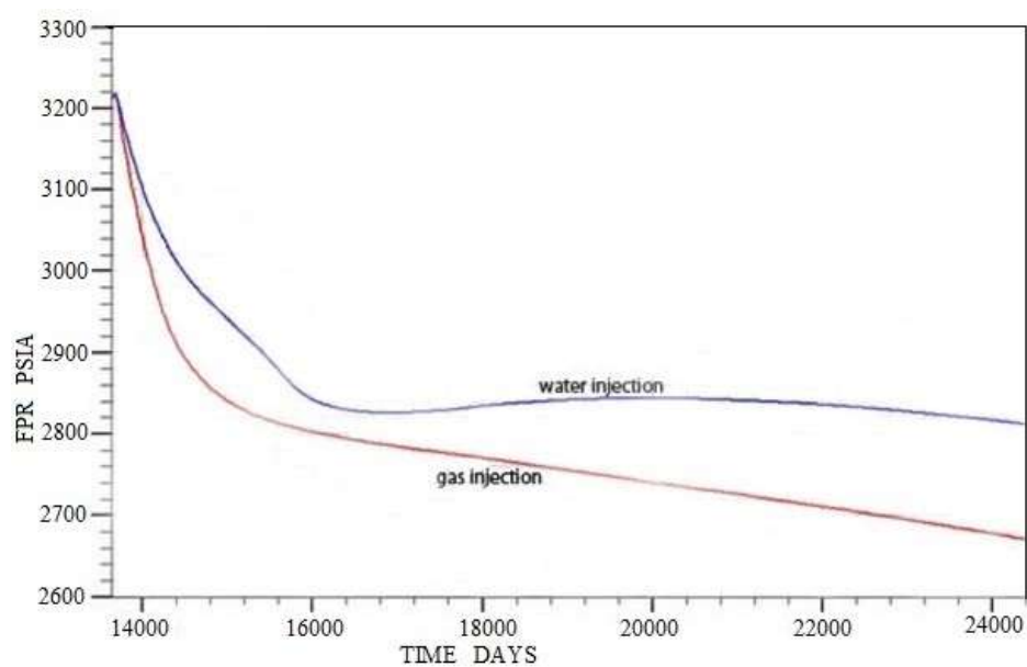
Figure.7. Comparison of Average Field Pressure for Two Scenarios.
