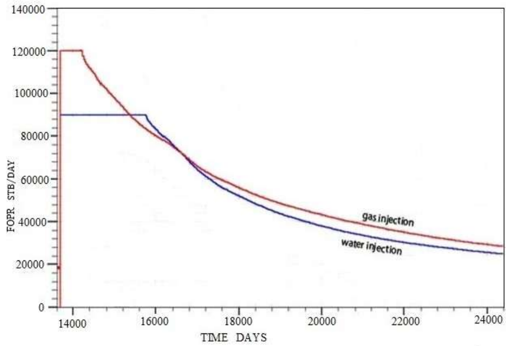
Figure.1. Comparison of Oil Production Rate for Two Scenarios.
