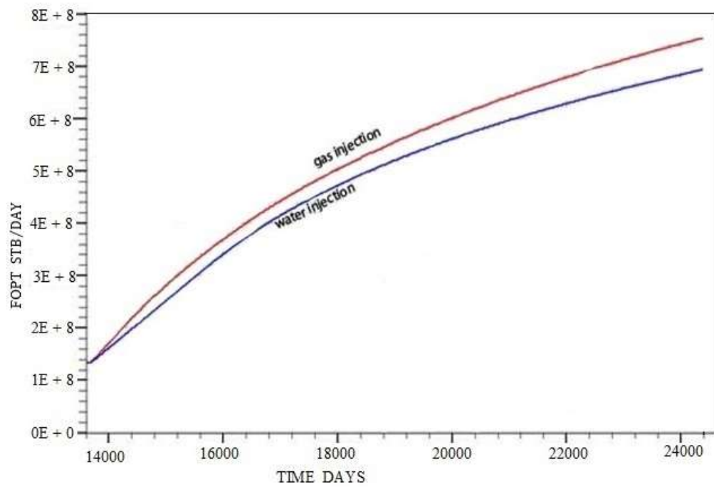
Figure.2. Comparison of Total Oil Production for two Scenarios.
