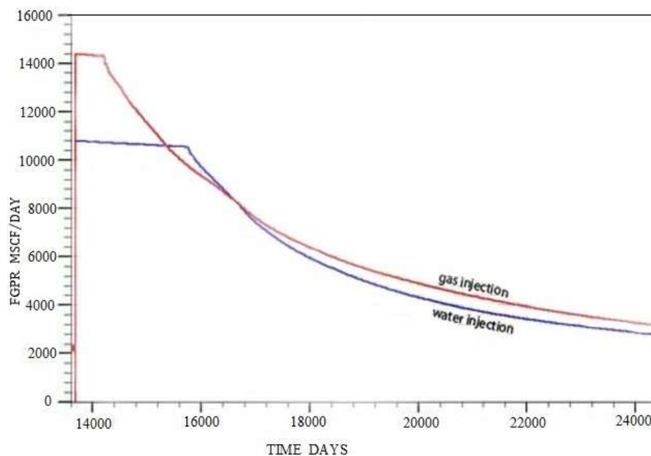
Figure.3. Comparison of Gas Production Rate for Two Scenarios.
