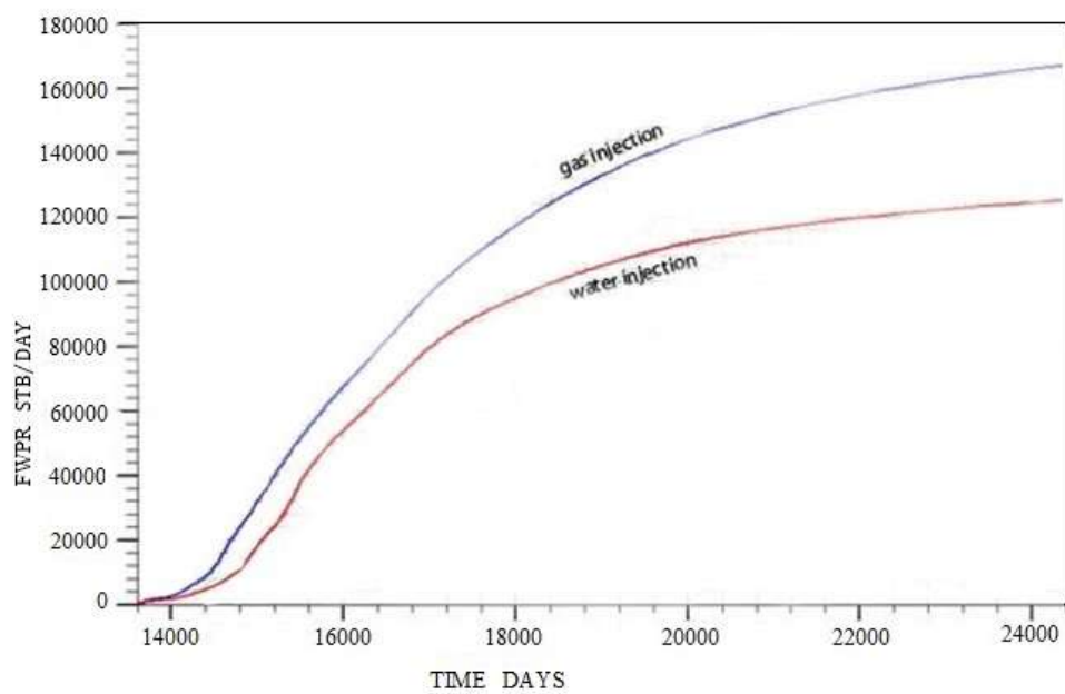
Figure.4. Comparison of Water Production Rate for Two Scenarios.
