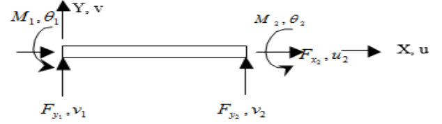
Figure 1 : Element beam in local coordinates
