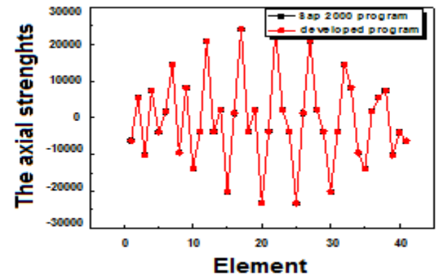
Figure 11 : Variation of the axial strength
