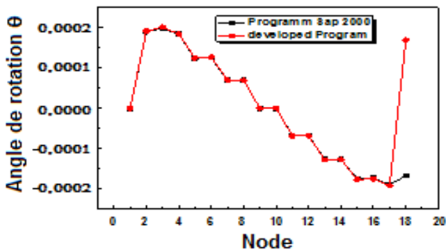
Figure 9 : Displacements in term of the rotation angle \theta
